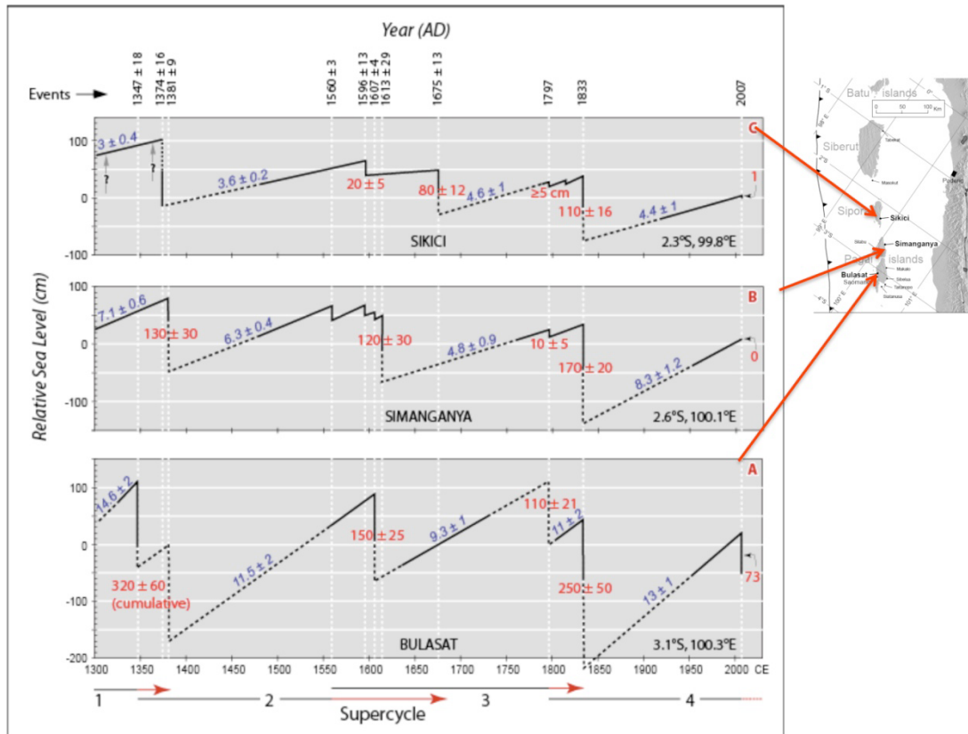
Graph of earthquake cycles in the Mentawai islands
