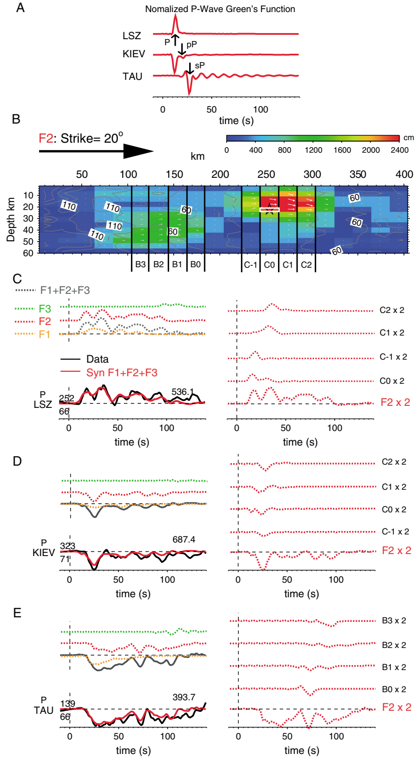
Figure 10. Representative teleseismic fits for stations at azimuth of 250°, 320°, and 140°. We selected three representative teleseismic stations (LSZ, KIEV, and TAU) from three groups of stations (Boxes) as indicated in Figure 9 for detailed modeling. An example of normalized Green's Functions for the three stations, direct P, and ocean bottom reflection pP and sP phases are indicated by arrows in (A). The Green's Functions are computed by using unit slip on the subfault where the rupture on F2 was initiated, as shown in Figure 10B by the small white rectangle along with the slip model on fault segment F2. The rupture on this fault is divided into columns with corresponding synthetics presented in Figures 10C, 10D, and 10E. (C) Lower left shows the entire waveform fit at station LSZ, synthetic is decomposed into the contribution of fault segments F1, F2, and F3 as displayed on upper left. The panel on the right panel shows the contribution of columns C-1 to C2 on F2. Figures 10D and 10E are similar as Figure 10C for stations KIEV and TAU.
