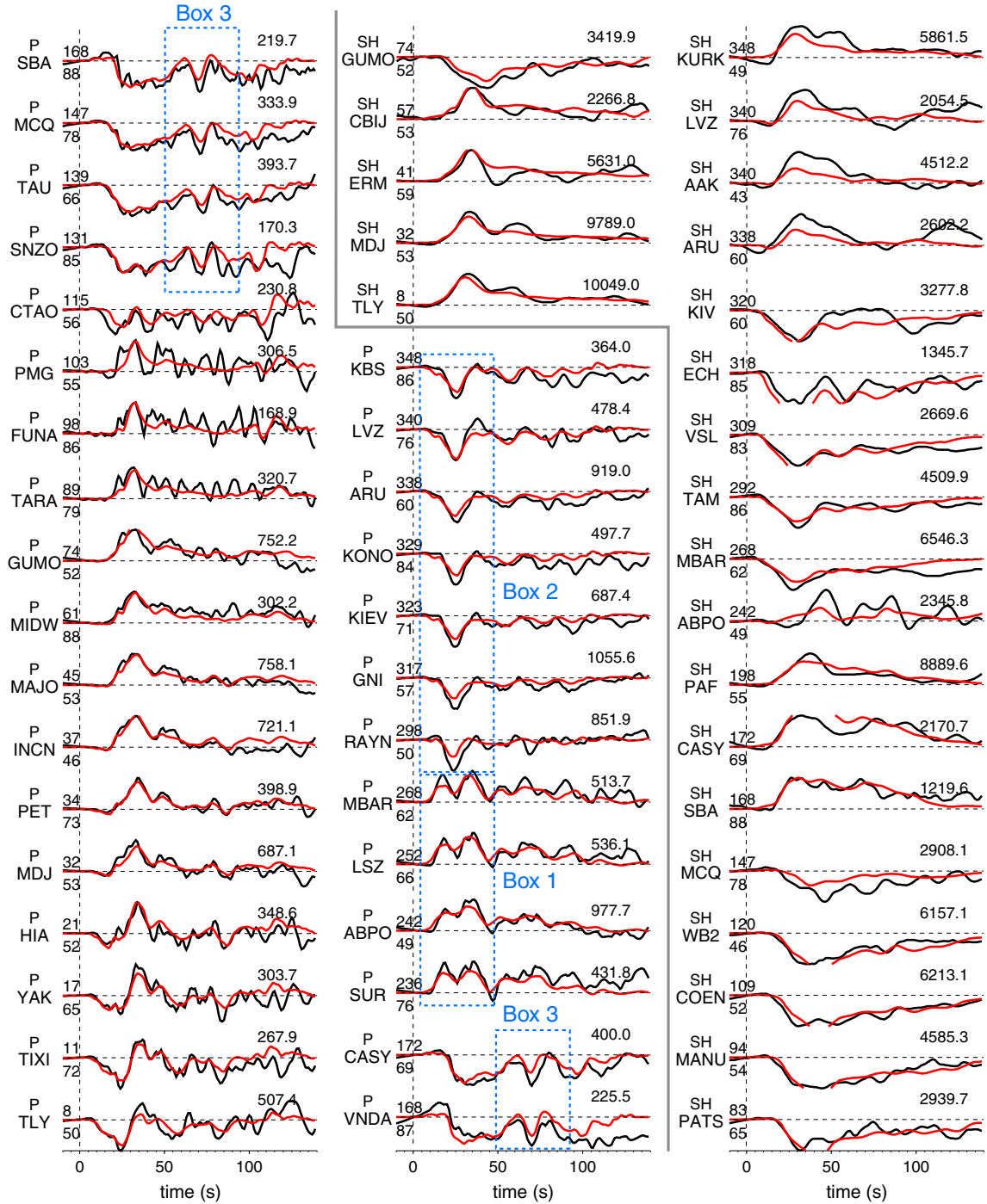
Figure 9. Telesismic waveform fits. The telesismic waveform fits for the joint inversion model are presented where P and SH waves are separated by the heavy gray line. The data are displayed in black and synthetics in red; the station name is indicated at the beginning of each trace with epicenter distance in degree (lower) and azimuth (upper). The maximum amplitudes of data in micrometers are shown at the end of the seismograms. Stations at three azimuths groups are indicated by the dashed rectangles (Box1, Box2, and Box3) with representative stations shown in Figure 10.
