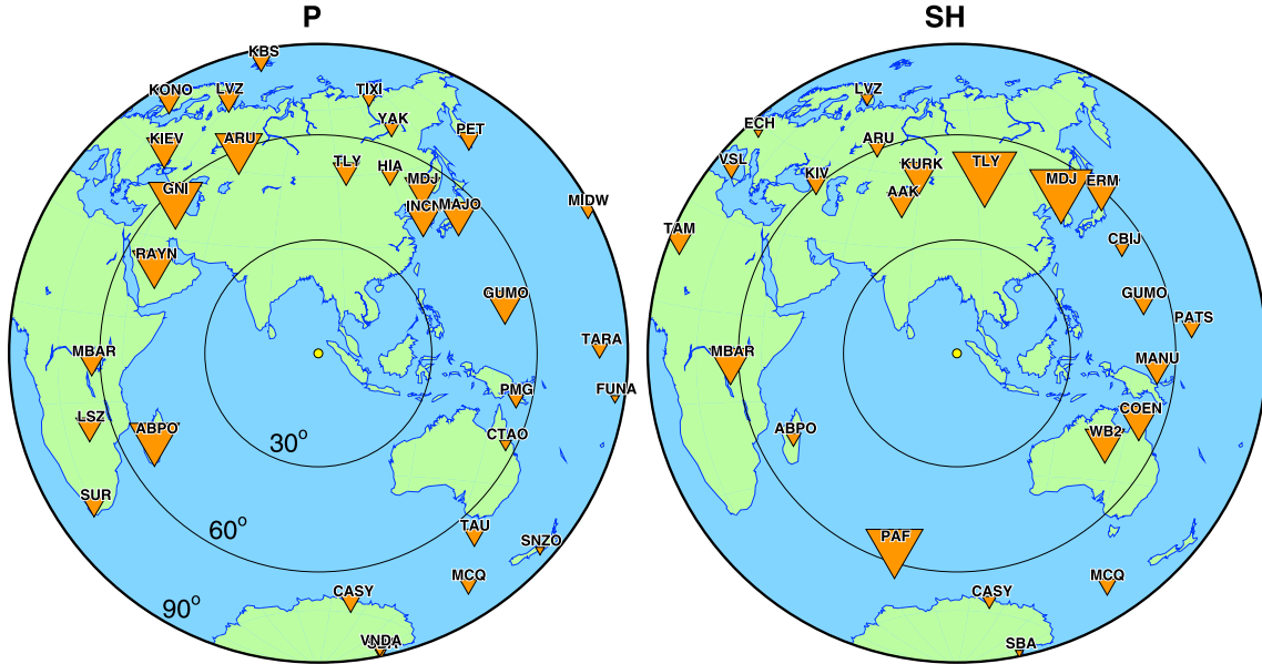
Figure 6. Telesismic station map. The station distribution of telesismic P and SH components used in the inversions where the size of triangle is proportional to the maximum displacement amplitude for each station. Note that the largest amplitude directions between the P and SH waves are rotated by 45^\circ as predicted for a strike-slip event.
